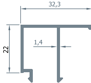
1986 CAM ÇİTASI 0.266 kg/m.
