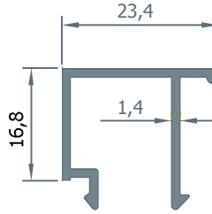
1986 CAM ÇİTASI 0.266 kg/m.
