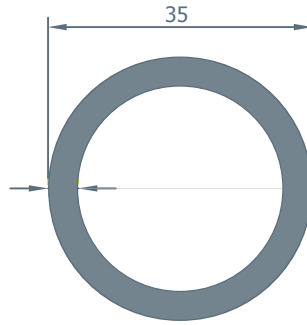
516 1.056 kg/m.
