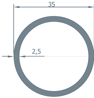
612 0.692 kg/m.
