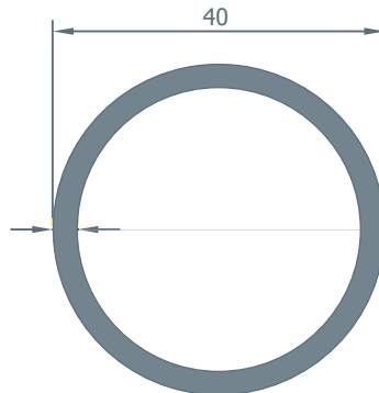
515 0.945 kg/m.
