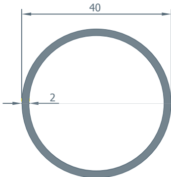
613 0.648 kg/m.
