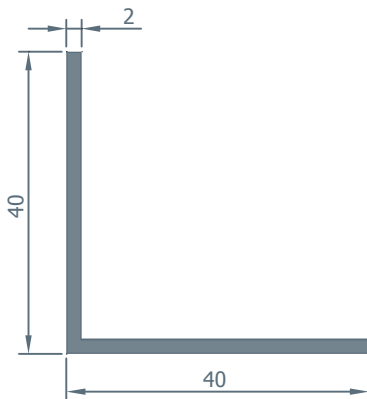
601.13 0.423 kg/m.
