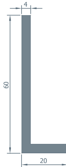
601.18 0.824 kg/m.
