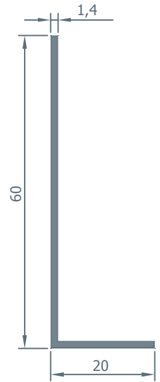
4665 0.298 kg/m.
