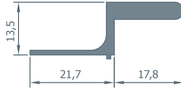
2962 0.355 kg/m.
