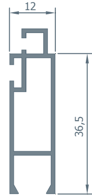
2543 0.380 kg/m.
