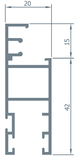
2086 0.607 kg/m.
