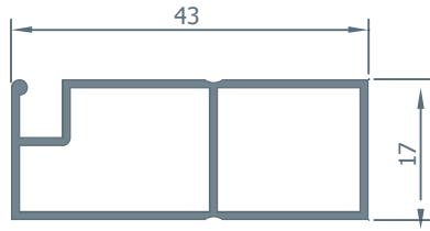
2050 0.410 kg/m.
