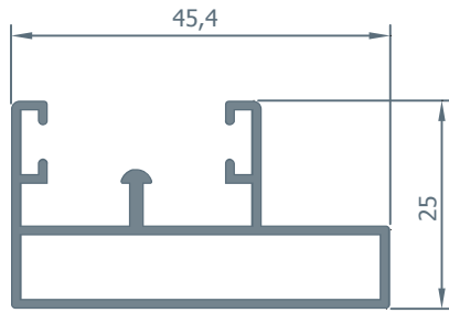
2314 0.542 kg/m.
