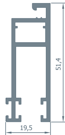
4462 0.780 kg/m.
