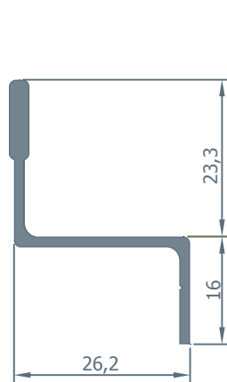
2026 0.322 kg/m.
