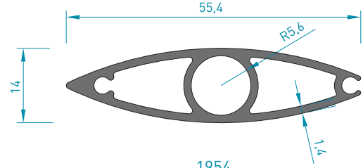
1954 YAPRAK PROFİL 0.560 kg/mt
