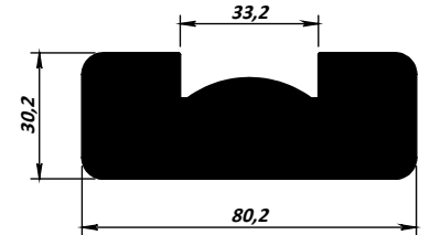
MK-61 - 5,792 kg/m
