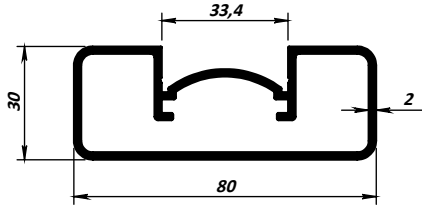
MK-30 - 1,360 kg/m
