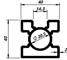
MK-33 - 1,255 kg/m
