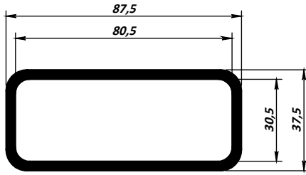
MK-62 - 2,163 kg/m
