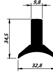
MK-38 - 1,052 kg/m
