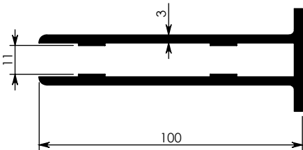
7694 - 2,000 kg/m
