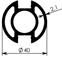
MK-21-D - 1,145 kg/m
