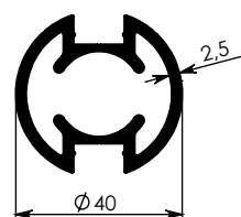
MK-23-D - 1,095 kg/m
