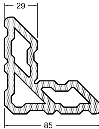
5680-29 5.697 kg/m
