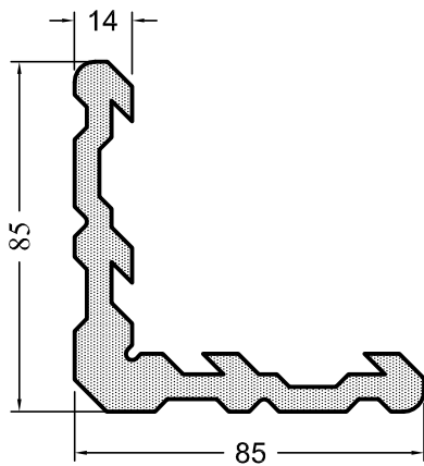
5680-14 3.922 kg/m
