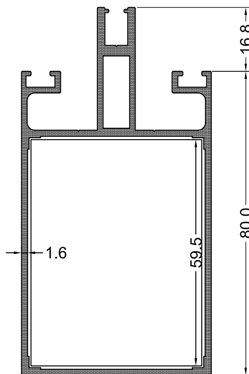
AG 701 I_x = 54.47 1,600 Kg/m I_y = 19.53
