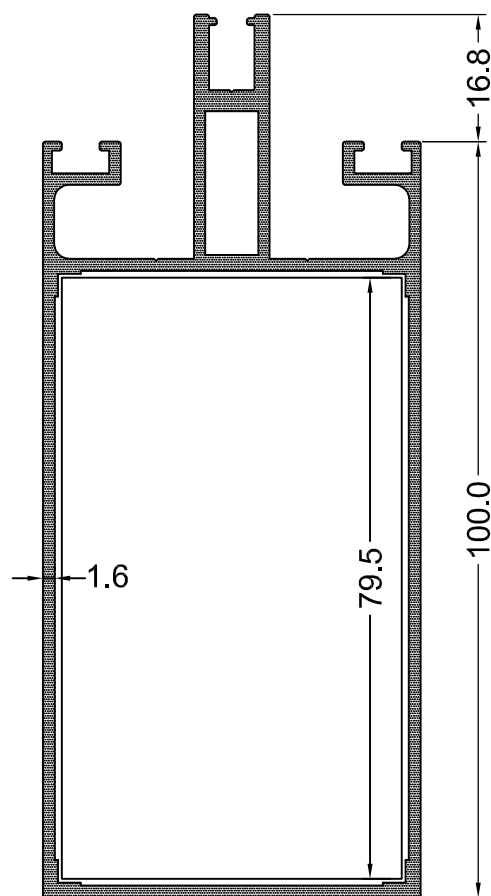
AG 737 I_x = 91.97 1,630 Kg / m I_y = 23.58
