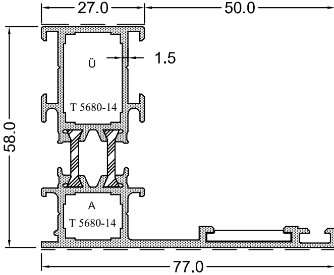
GKS 58-01 1.433 Kg/m
