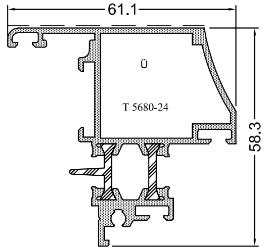
GKS 58-31 1.251 Kg/m
