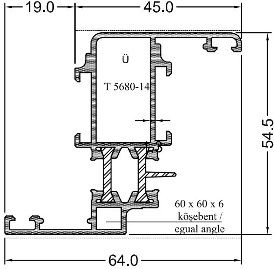
EY4534-13 1.083 Kg/m I_x = 3.42 I_y = 16.01
