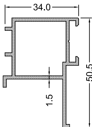
GKS 58-50 0.620 Kg/m
