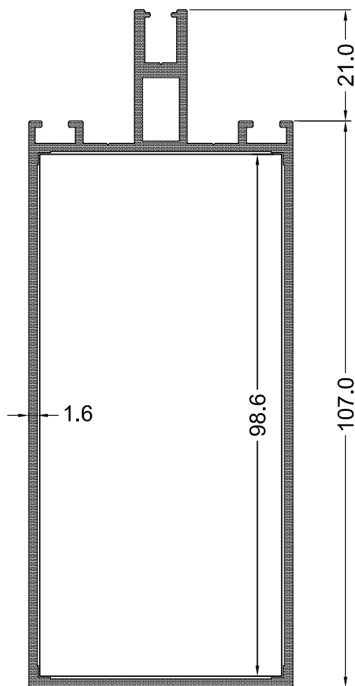
AG 755 I_x = 110.97 1,683 Kg / m I_y = 23.50
