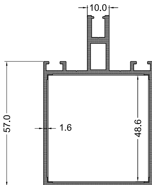
AG 757 1,250 Kg / m I_x = 23.36 I_y = 14.13
