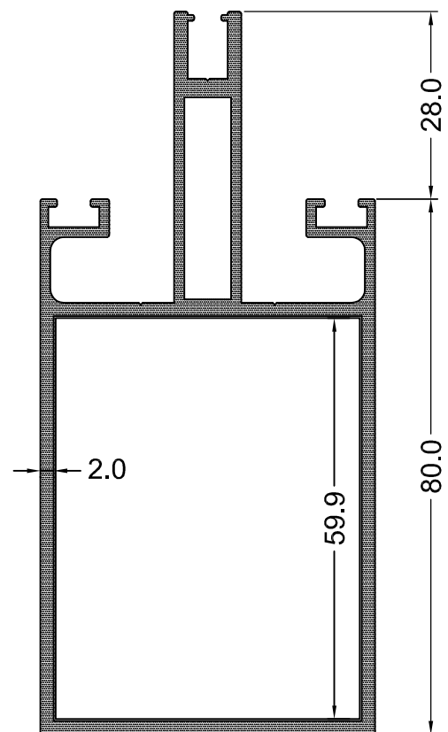
AG 706 - (1696) I_x = 73.12 1,930 Kg / m I_y = 22.67
