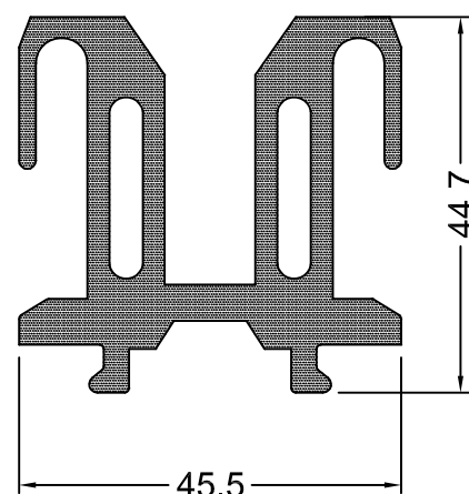
AG-745 2,160 Kg/m
