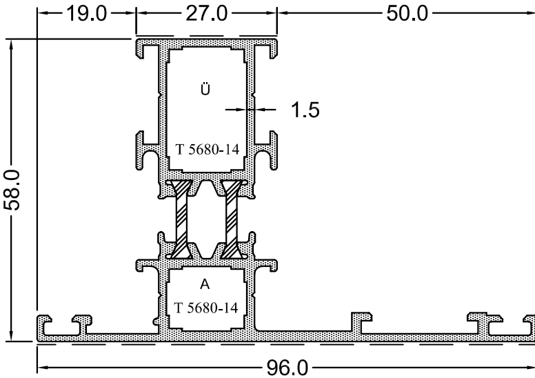
GKS 58-02 1.541 Kg/m
