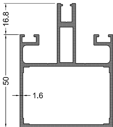
AG 738 I_x = 19.11 1,195 Kg/m I_y = 14.21
