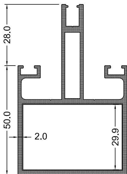
AG 708-(2393) I_x = 28.73 1,605 Kg / m I_y = 15.75
