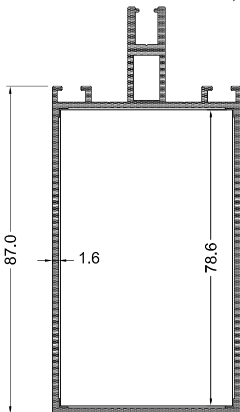
AG 756 I_x = 69.82 1,510 Kg / m I_y = 19.75
