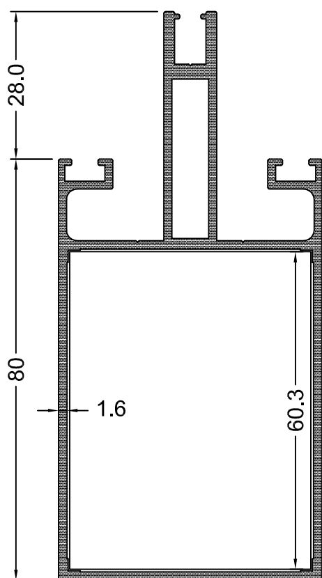
AG 707 - (2761) I_x = 65.25 1,692 Kg / m I_y = 19.58
