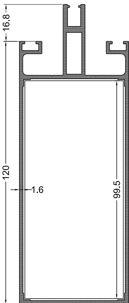
AG 700 I_x = 142.25 1,950 Kg/m I_y = 27.33
