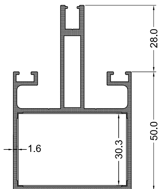
AG 709 - (2762) I_x = 26.10 1,433 Kg / m I_y = 13.95
