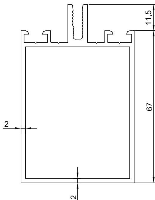
ALS-04 1,488 kg/m Jx:37,37 Jy:19,01
