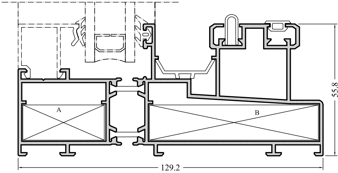
AS-111 2,474 kg/m
