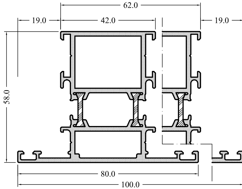
Y5821-20 1,825 kg/m
