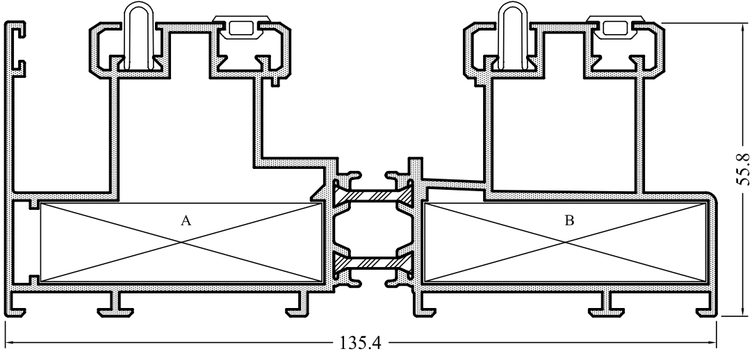
AS-110 2,960 kg/m
