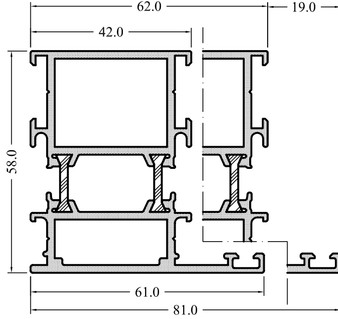
Y5802-20 1,710 kg/m
