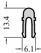
ALÜMİNYUM RAY AS - 160 0.125 Kg/m
