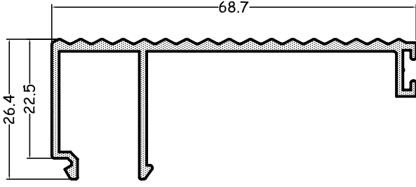
AS-155 0,585 kg/m
