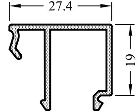
5644-15 0.315 Kg/m
