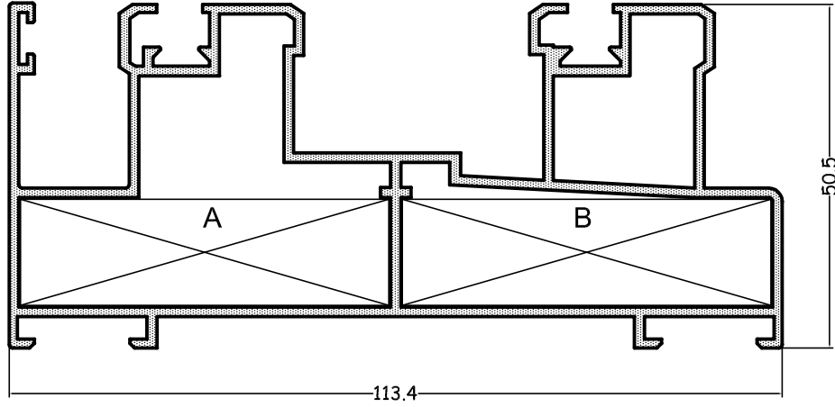
EL47-02 1,951 kg/m
