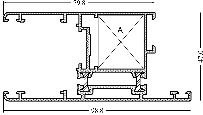
EL47-31 1,714 kg/m
